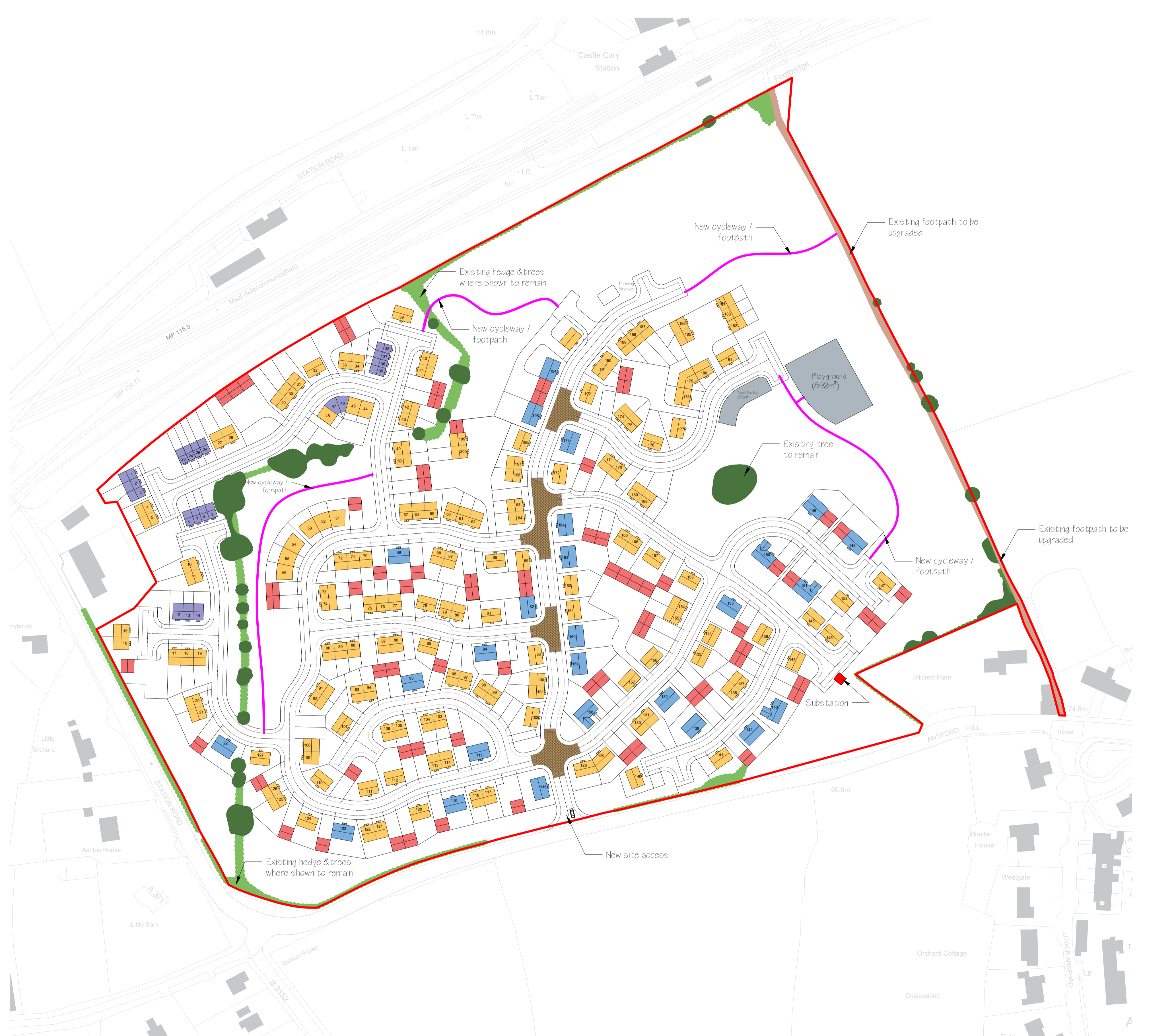
Proposed Housing Layout Plan - Scale 1:1000
